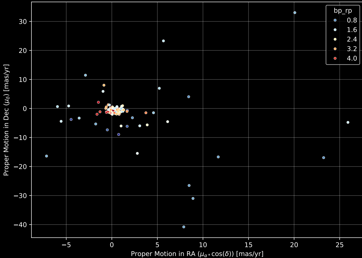
APOGEE DR17 Field: [ORIONA-E] Proper Motion Diagram (n= 132)
