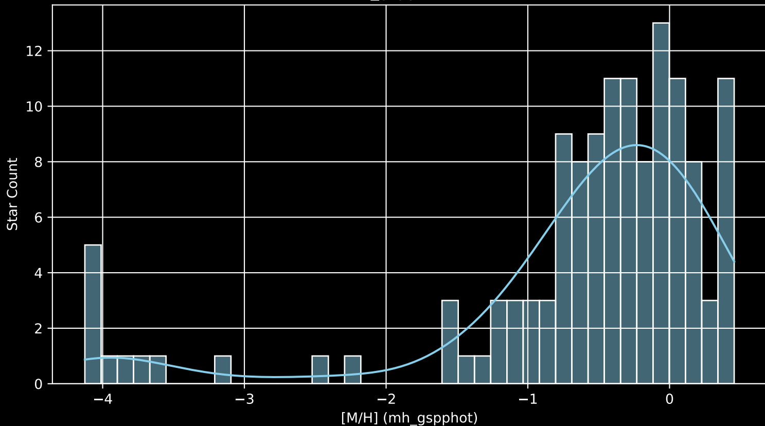
APOGEE DR17 Field: [ORIONA-E [M/H] (mh_gspphot) (n= 131)
