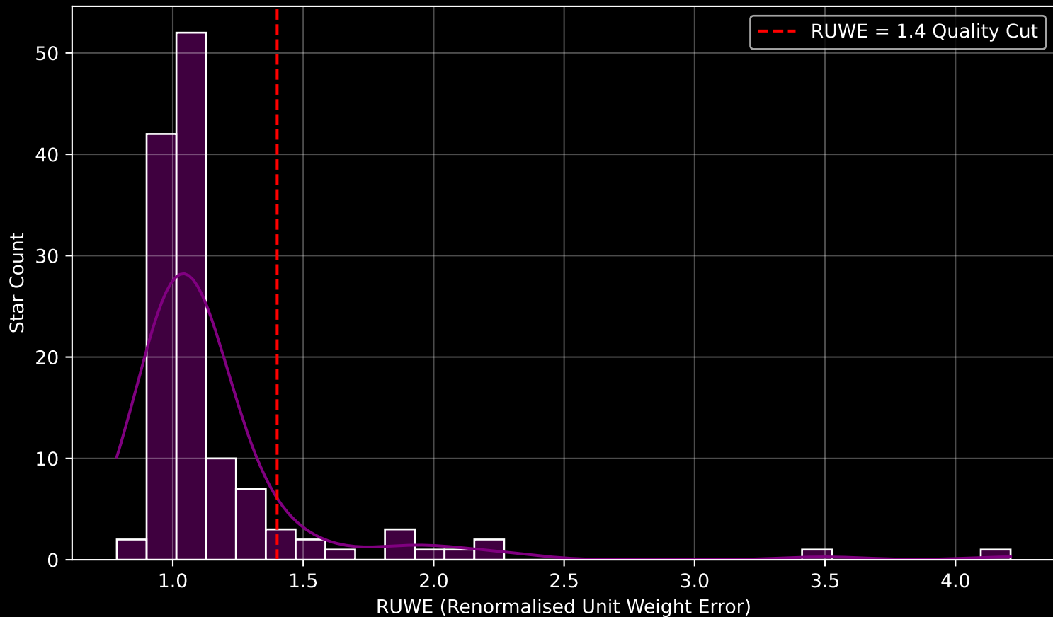
GAPOGEE DR17 Field [ORIONA-E] RUWE Distribution (n= 128)
