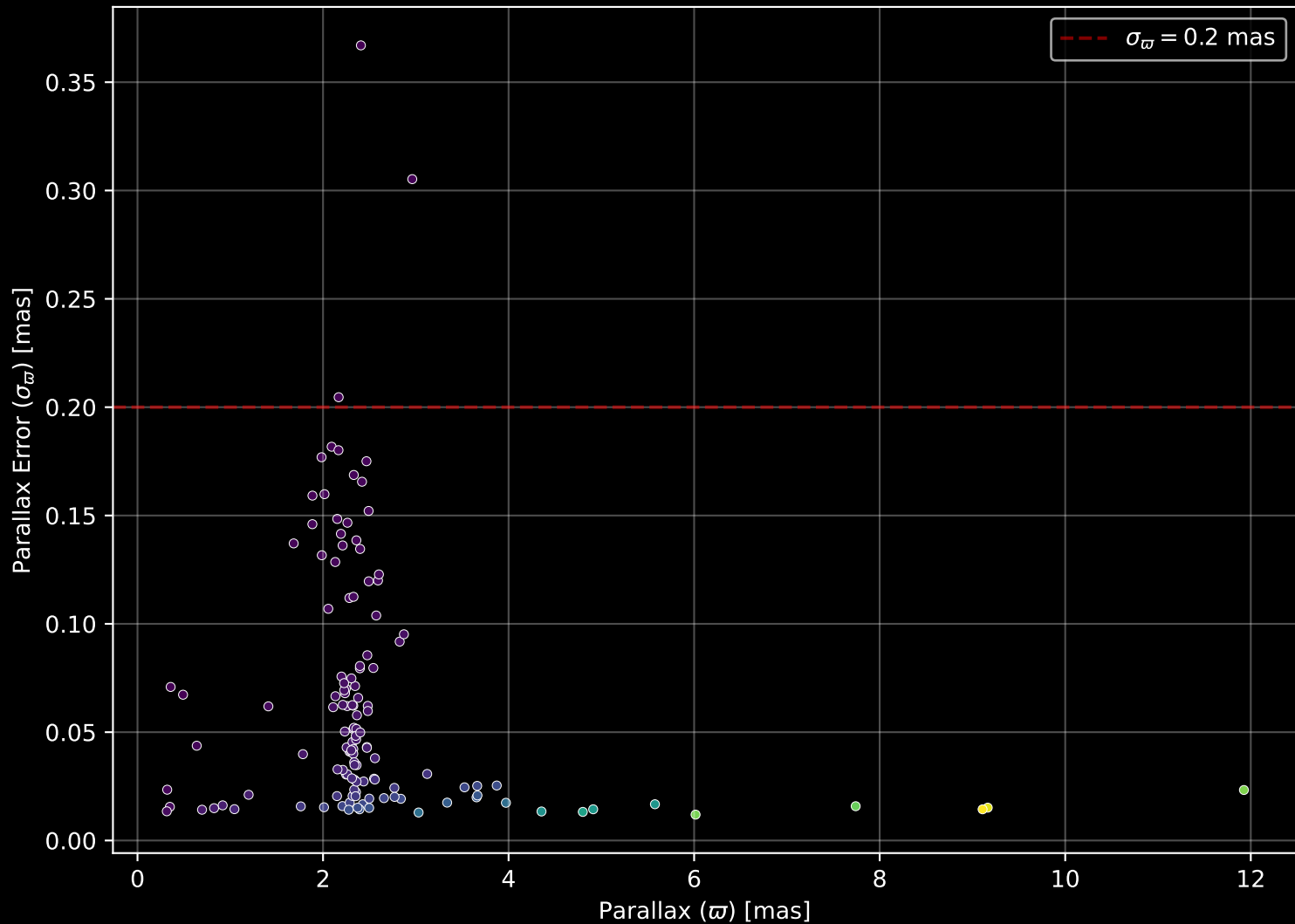
APOGEE DR17 Field: [ORIONA-E] Parallax Quality (n= 132)
